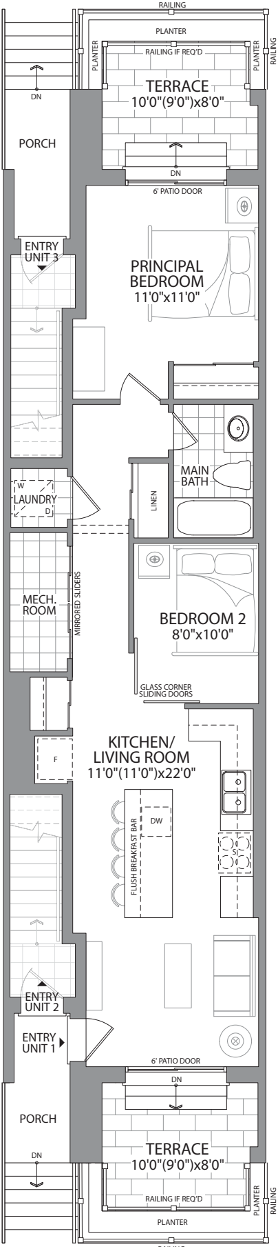
GROUND FLOOR
