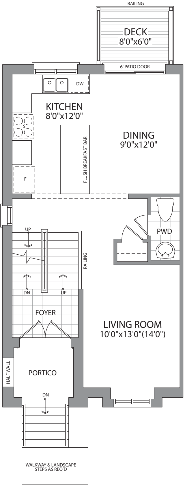
SECOND FLOOR
