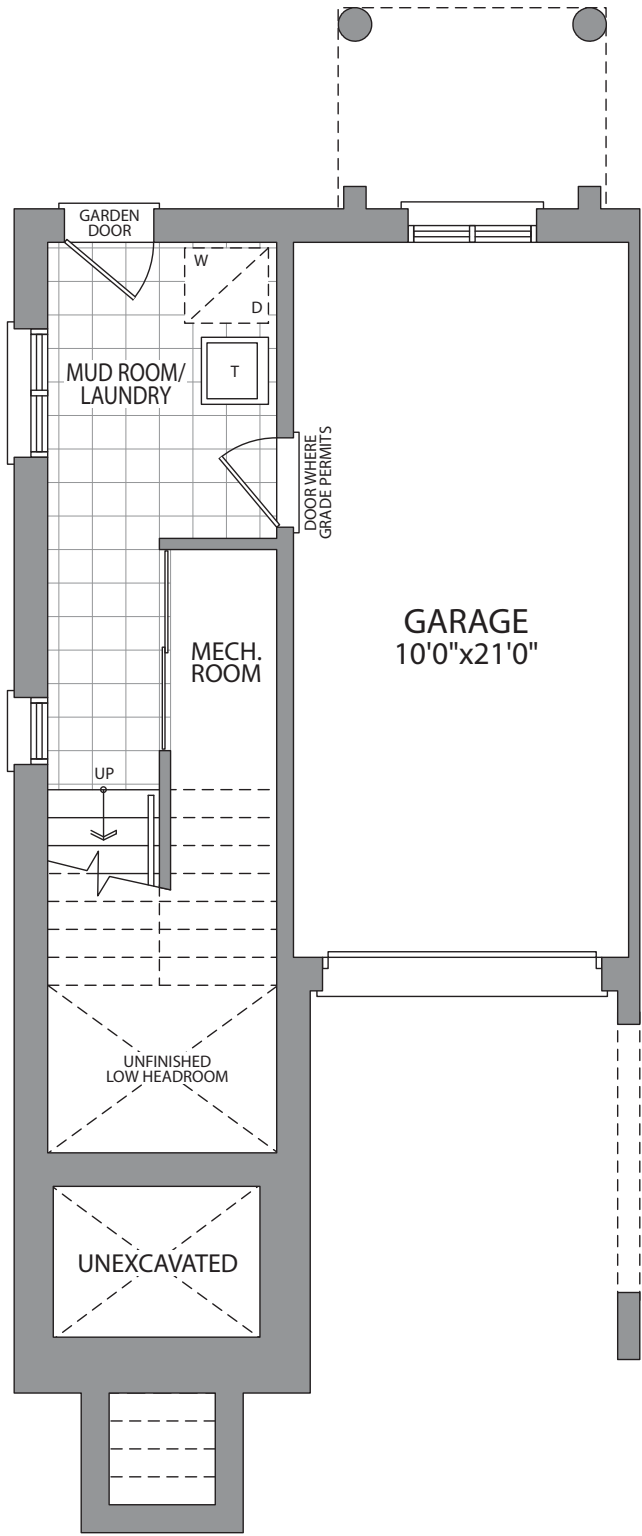
GROUND FLOOR
