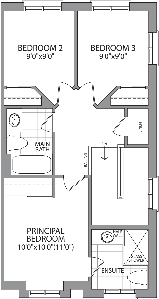
THIRD FLOOR
