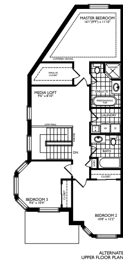
ALTERNATE UPPER FLOOR PLAN
