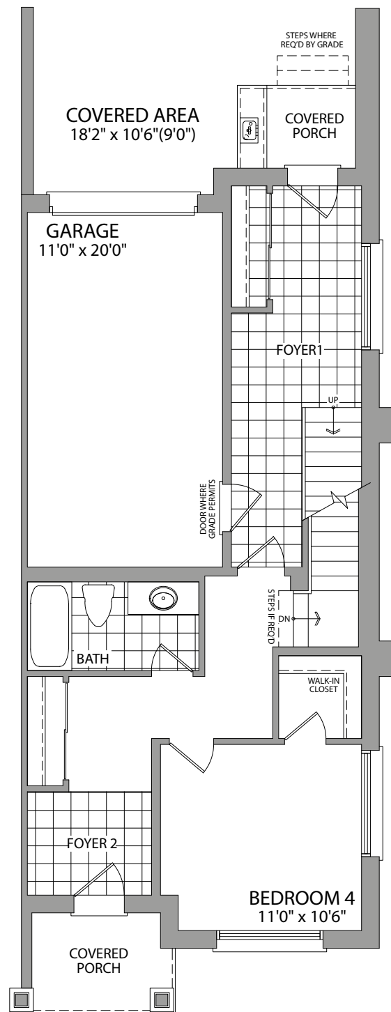
OPT. LOWER FLOOR ELEV. A END
