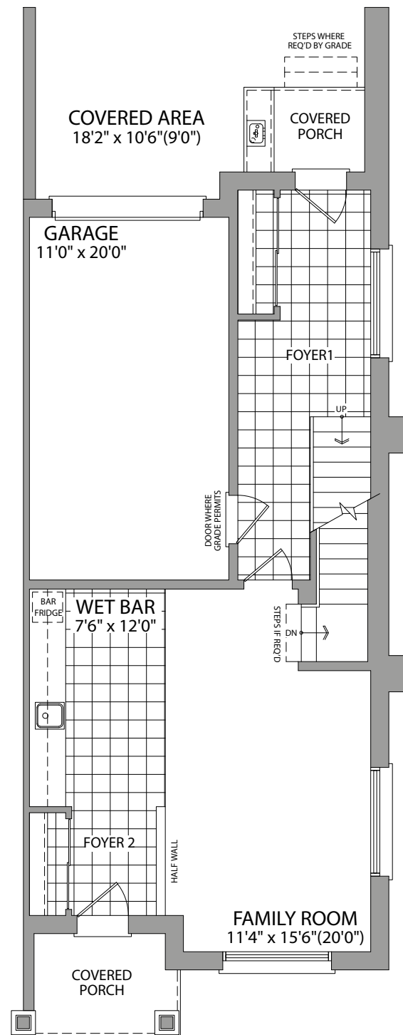
LOWER FLOOR ELEV. A END
