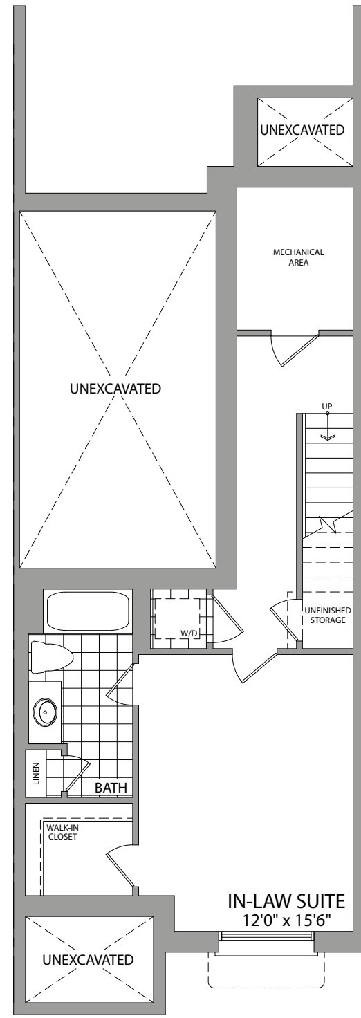
BASEMENT FLOOR ELEV. A1 & A2
